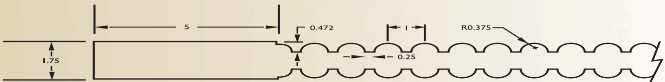
Standard Tambour Door Construction
