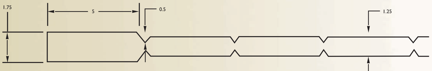
Standard V-Groove Door Construction
